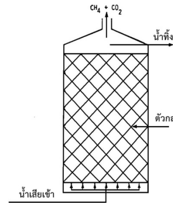
UPFLOW ANAEROBIC FILTER
